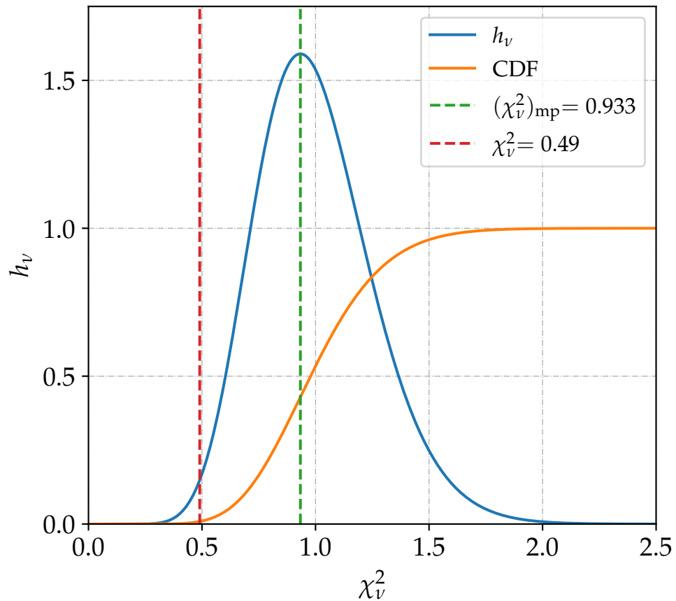
O\Lambda CDM
