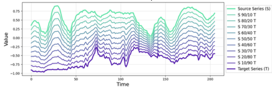
Linear Morph
