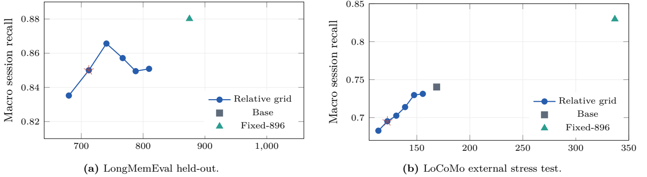
Figure 2: Macro evidence-session recall versus mean injected tokens. The policy frontier is corpus-dependent. The red star is the LongMemEval-selected RELATIVE-75 profile. It lies above-left of the LongMemEval base, but below-left of the LoCoMo base.
