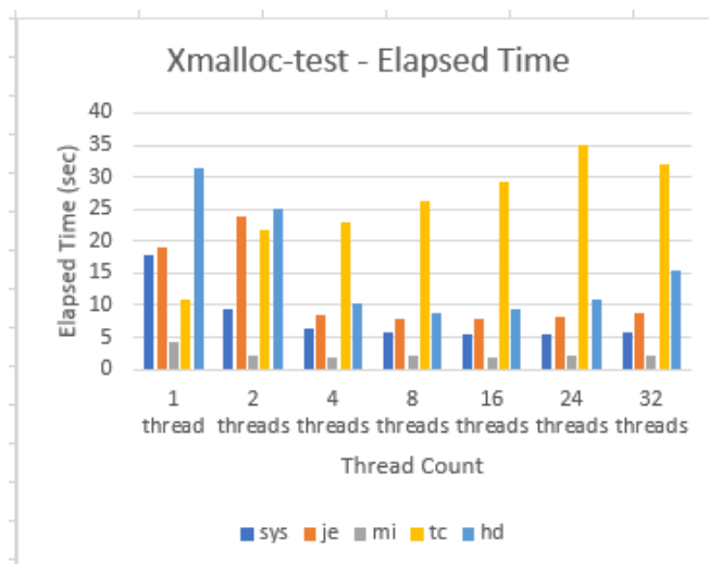
Figure 7. Mimalloc performs the best on the xmalloc-test benchmark. Tcmalloc starts well, but then struggles, while the rest spike before settling into reasonable runtimes.
