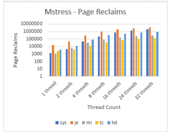
Figure 12. Despite its struggles with memory usage, mimalloc did better with page reclaims with the mstress benchmark. Jemalloc struggled, though. Note the log scale on the y axis.
