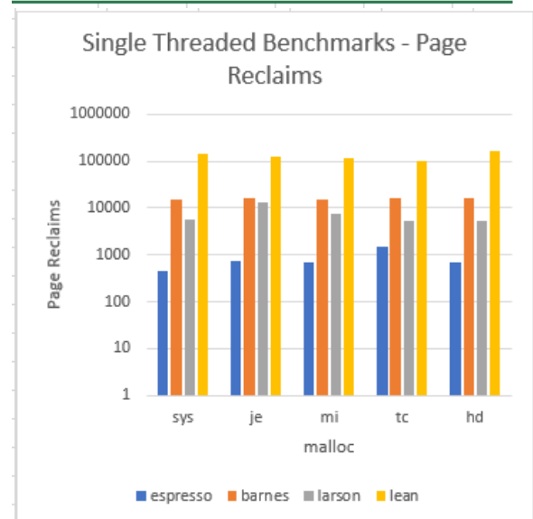
Figure 3. tcmmalloc showed some issues with page reclaims on a single thread, which may be due to its thread-local caches, which don't help it on a single thread. Note the log scale on the y axis. (Note that the larson benchmark data is corrupt - it is reported for completeness.)
