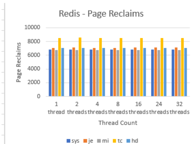
Figure 6. tcmalloc also performs the worst on page reclaims, a measure of how full the memory is, for the Redis benchmark. Again, the others perform similarly.
