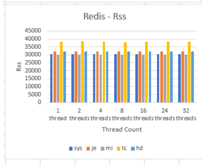
Figure 5. tcmalloc is the worst performer for resident set size (a measure of total memory usage) for Redis. The other allocators perform similarly across thread counts.
