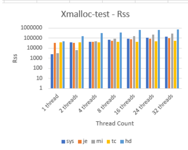
Figure 8. Hoard and mimalloc struggle more than expected with Rss on the xmalloc-test benchmark. Note the log scale on the y axis.
