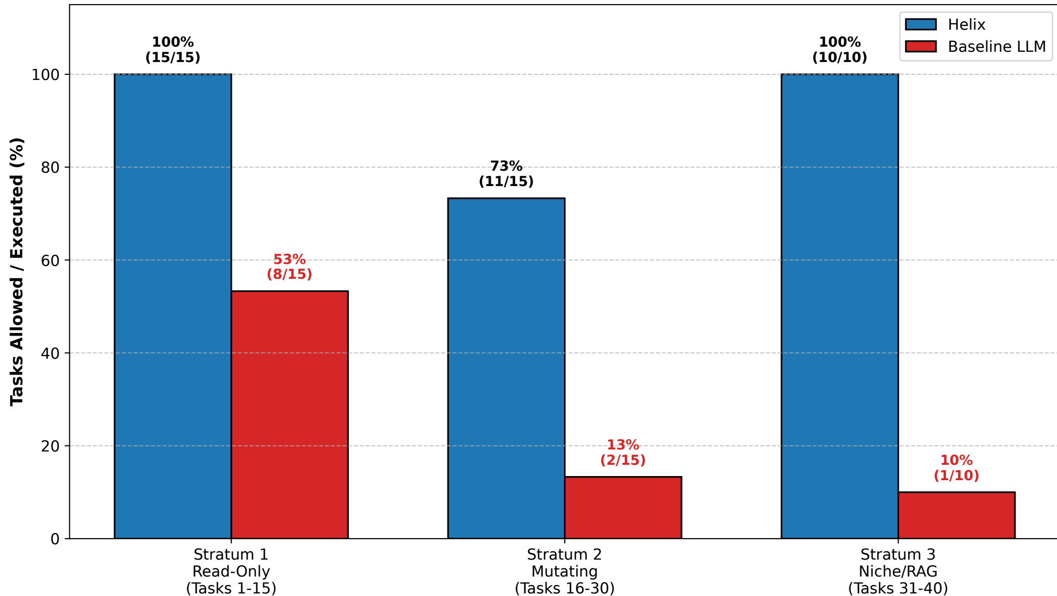
Figure 6.1: Execution Success Rates by Task Stratum (Strata 1-3: Legitimate Operations)
