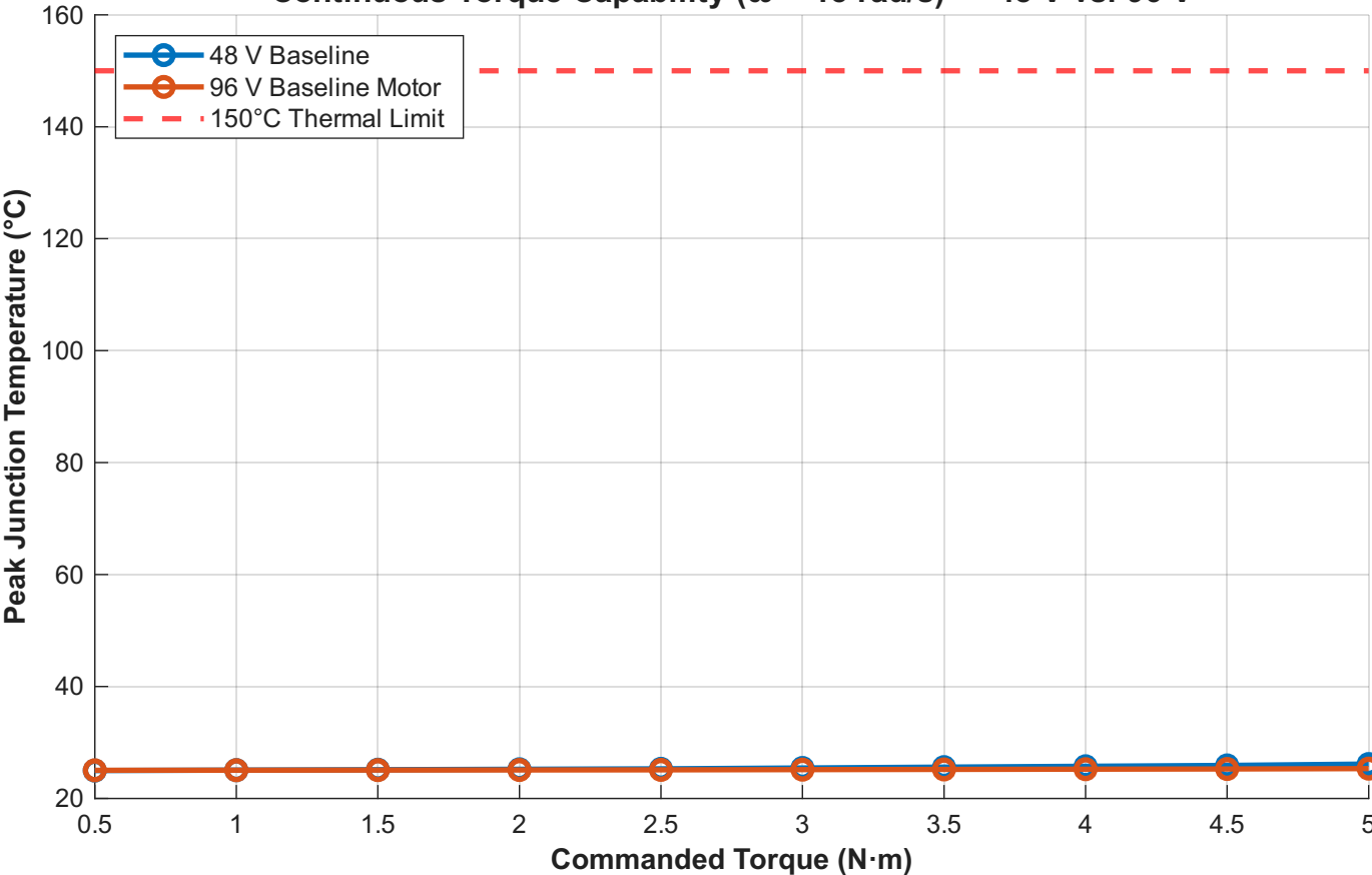
Continuous Torque Capability ( \omega = 15 \text{ rad/s} ) — 48 V vs. 96 V
