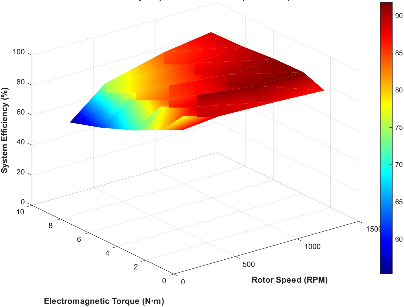
Efficiency Map — 48 V Baseline (Si, 40 kHz)
