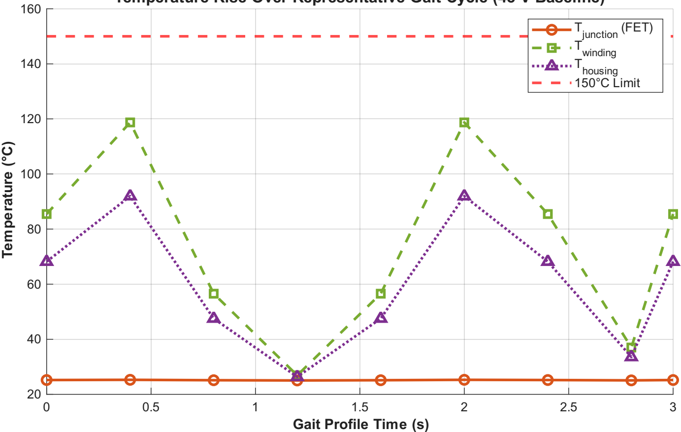
Temperature Rise Over Representative Gait Cycle (48 V Baseline)
