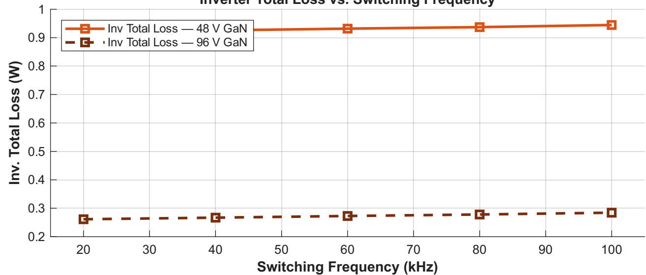
Inverter Total Loss vs. Switching Frequency
