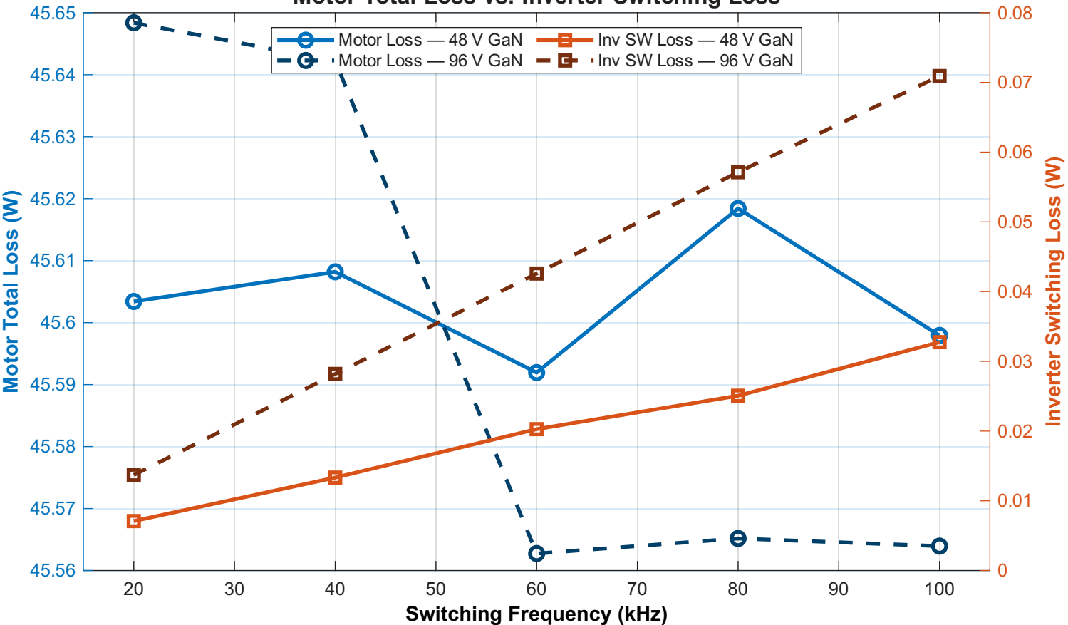
Motor Total Loss vs. Inverter Switching Loss
