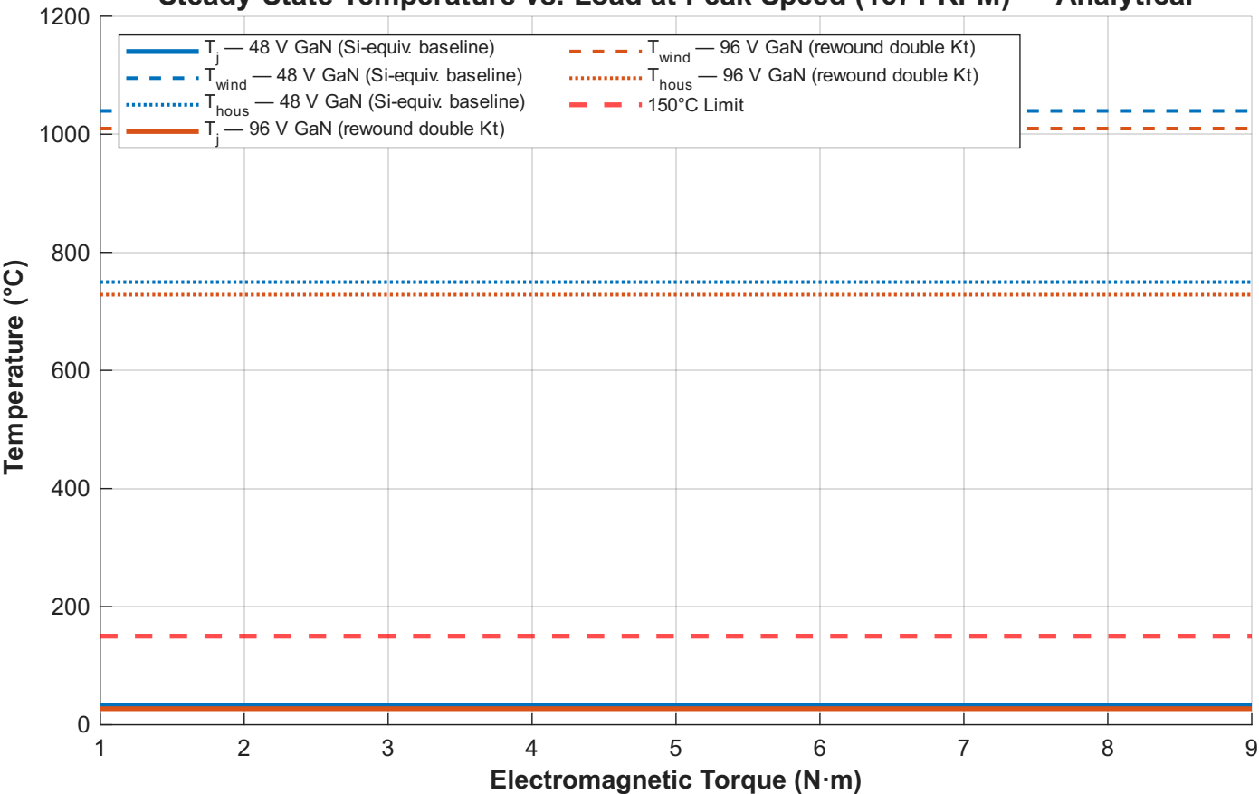
Steady-State Temperature vs. Load at Peak Speed (1671 RPM) — Analytical
