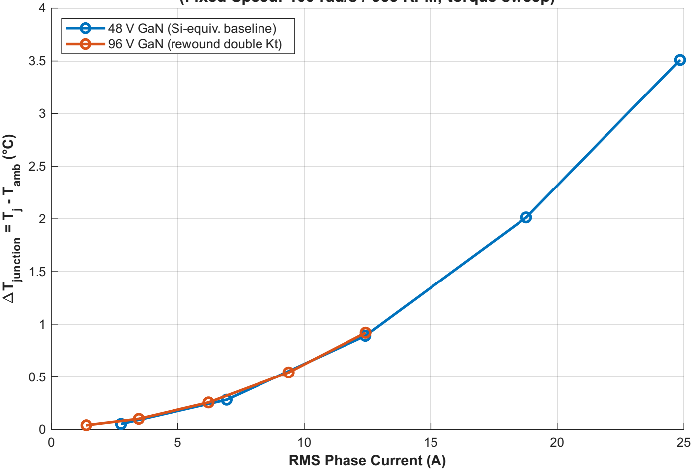
Junction Temperature Rise vs. RMS Phase Current (Fixed Speed: 100 rad/s / 955 RPM, torque sweep)
