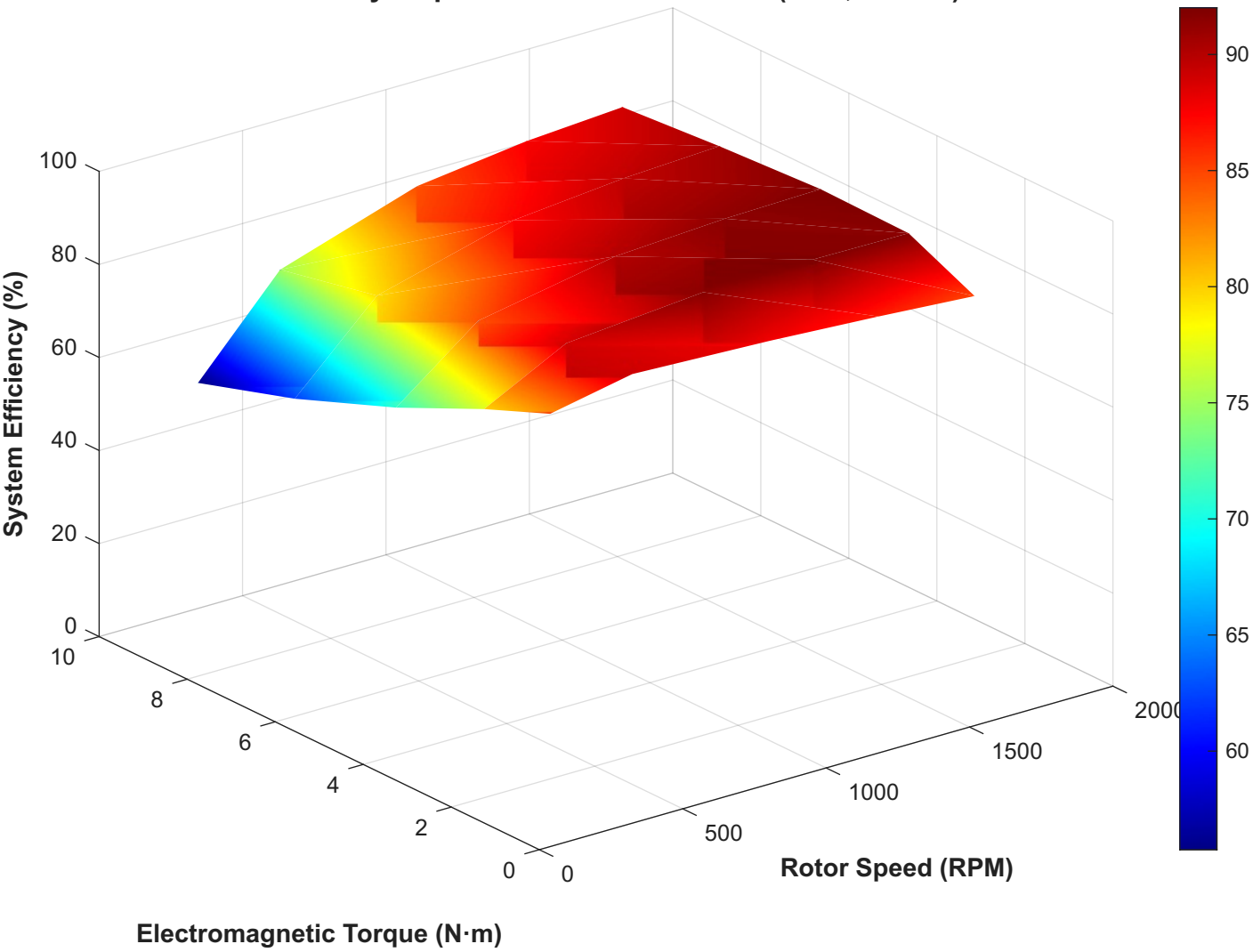
Efficiency Map — 96 V Baseline Motor (GaN, 40 kHz)
