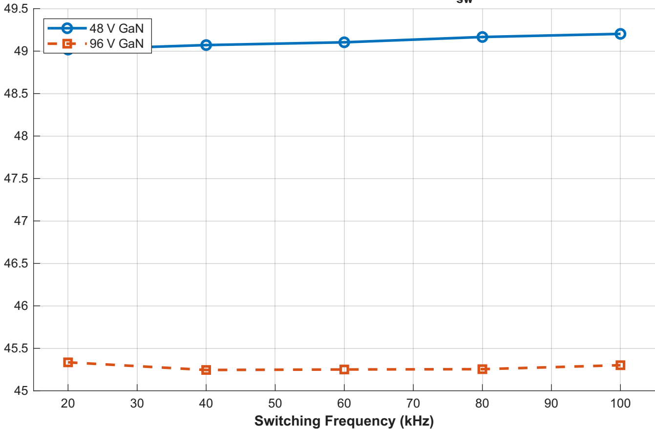
Switching-Frequency Sweep — Total Loss vs. f_{sw} (48 V vs. 96 V)
