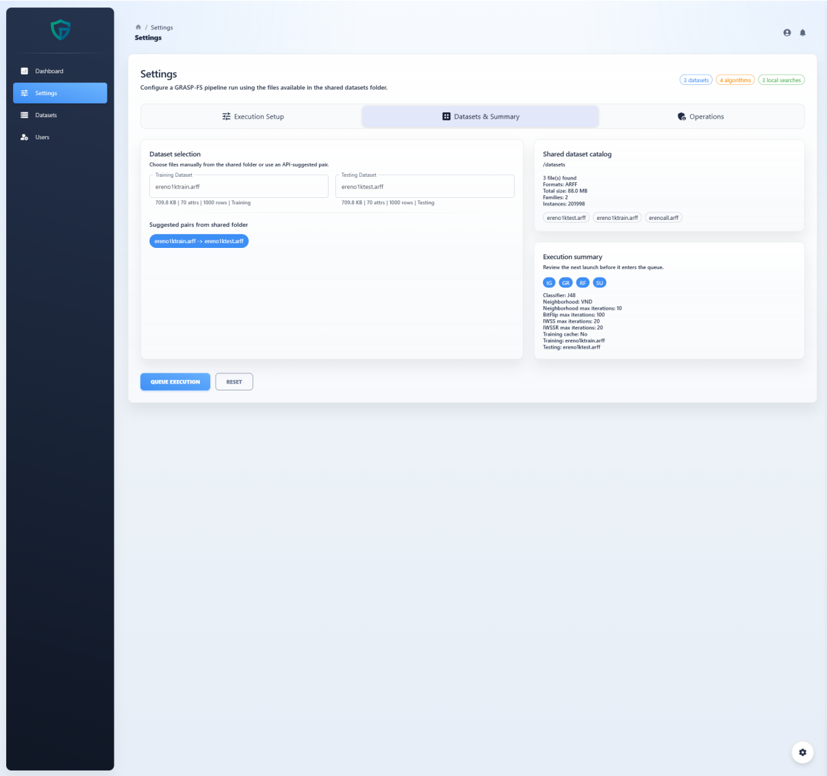
Figure 32 – Dataset settings.
