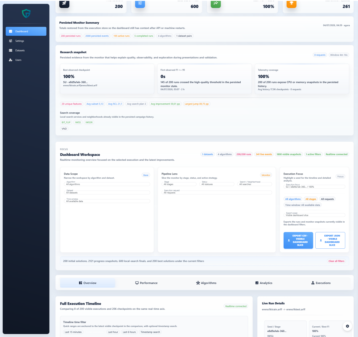
Figure 17 – Overview dashboard.
