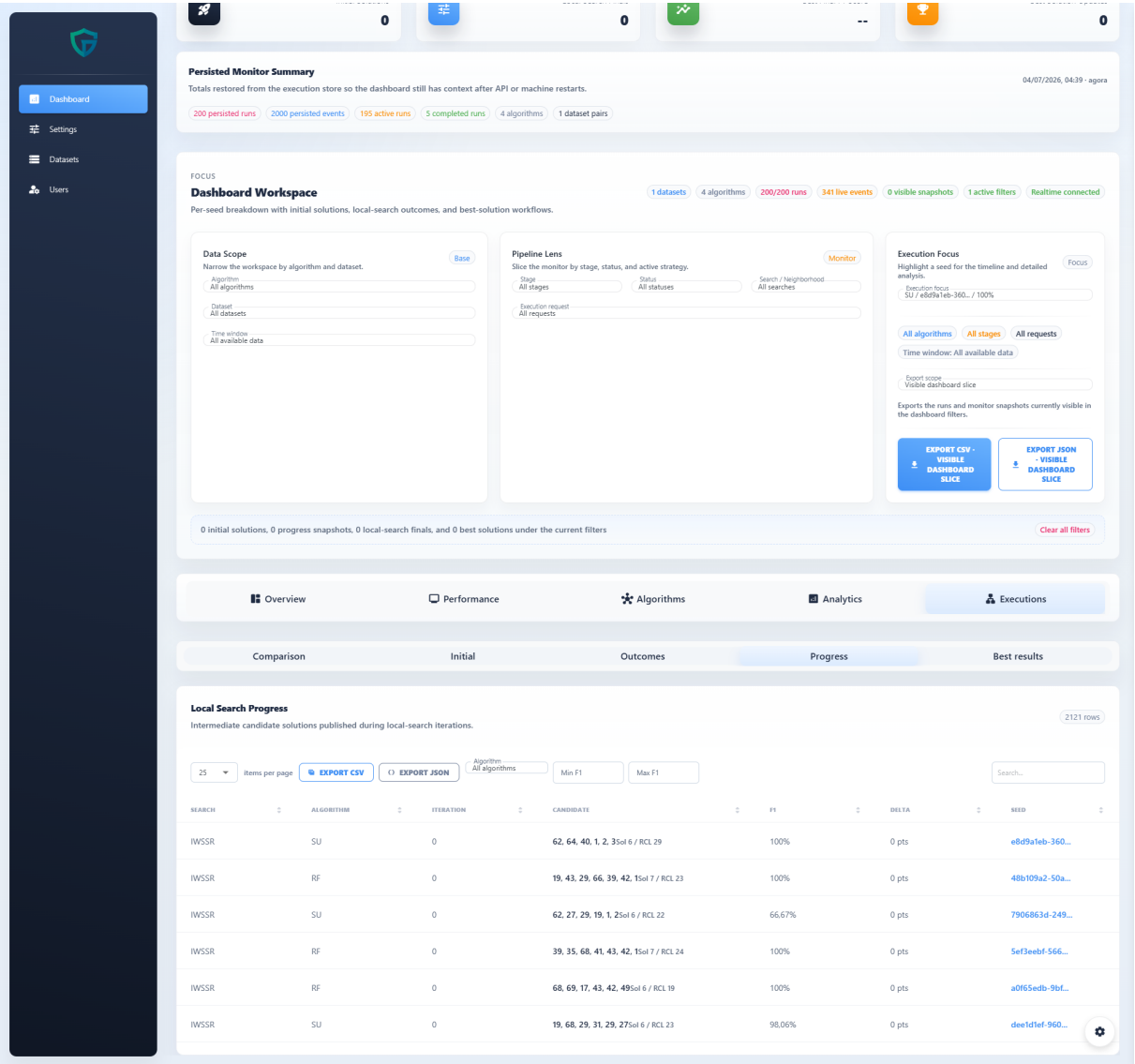
Figure 29 – Execution progress.
