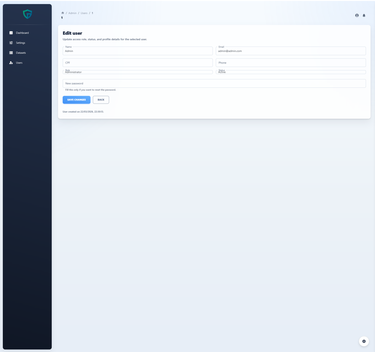
Figure 37 – User editing.
