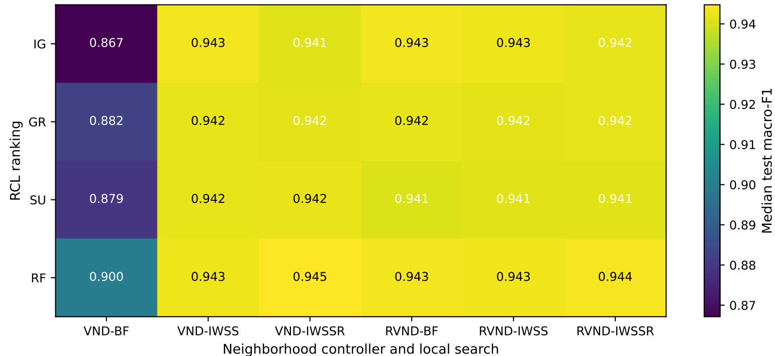
Median held-out macro-F1 for G-FShield configurations
