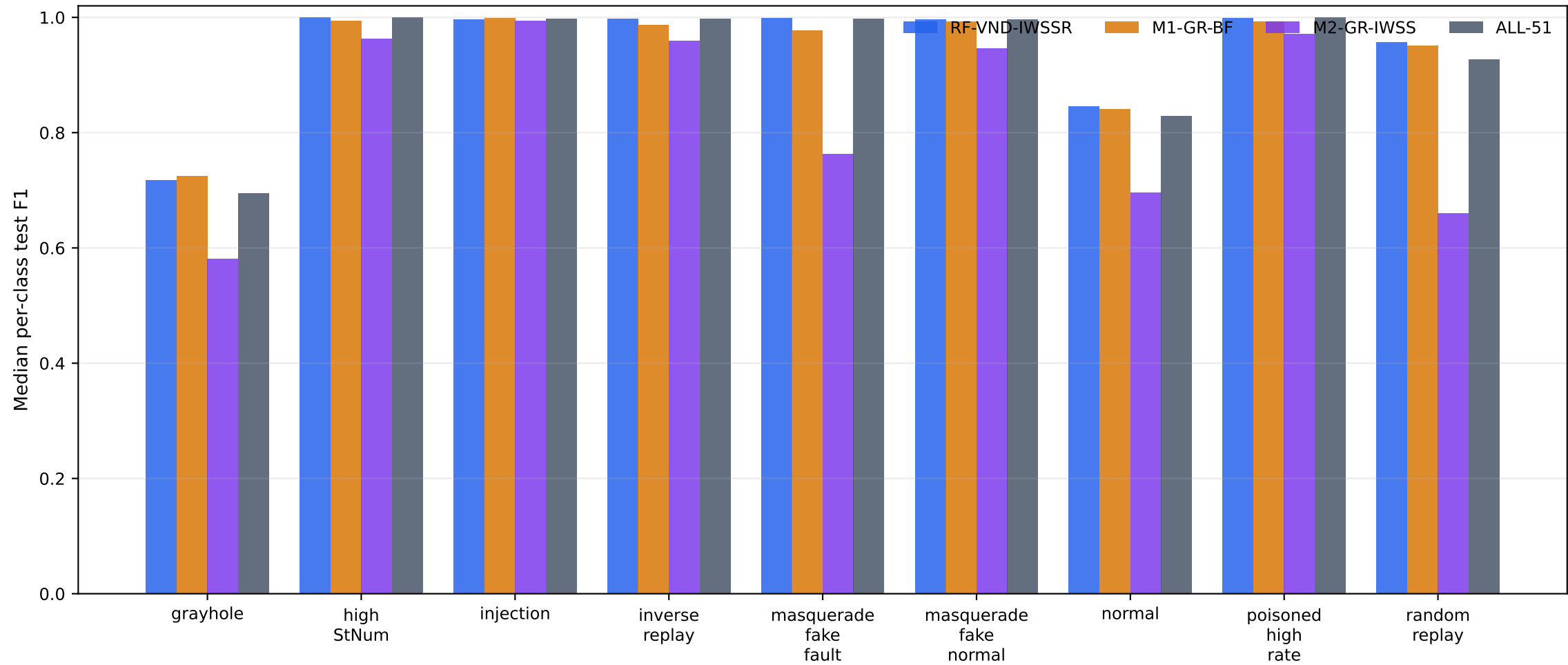
Held-out per-class performance of the validation-selected G-FShield configuration and comparators
