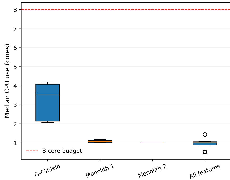
Observed container resources under the common aggregate budget
