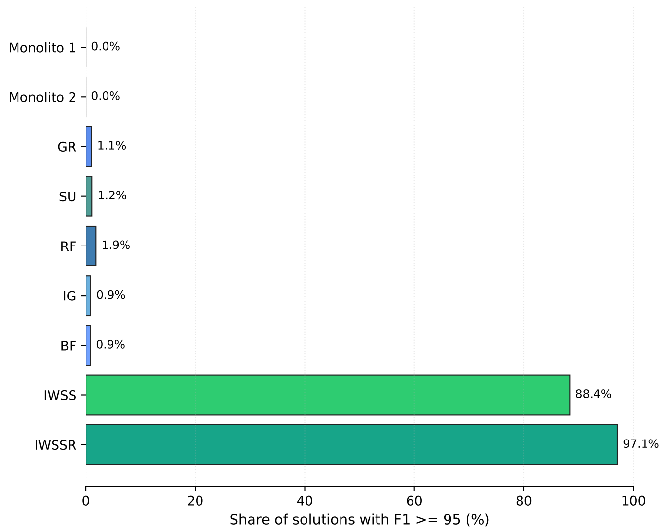
High-quality tail
