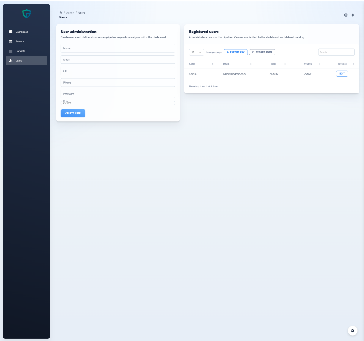
Figure 39 – User list.
