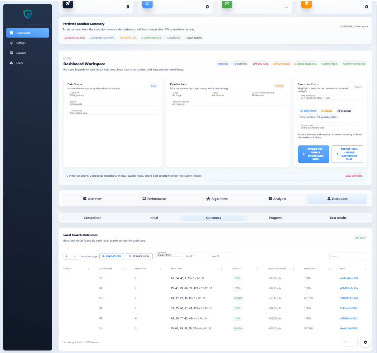
Figure 31 – Consolidated outcomes.
