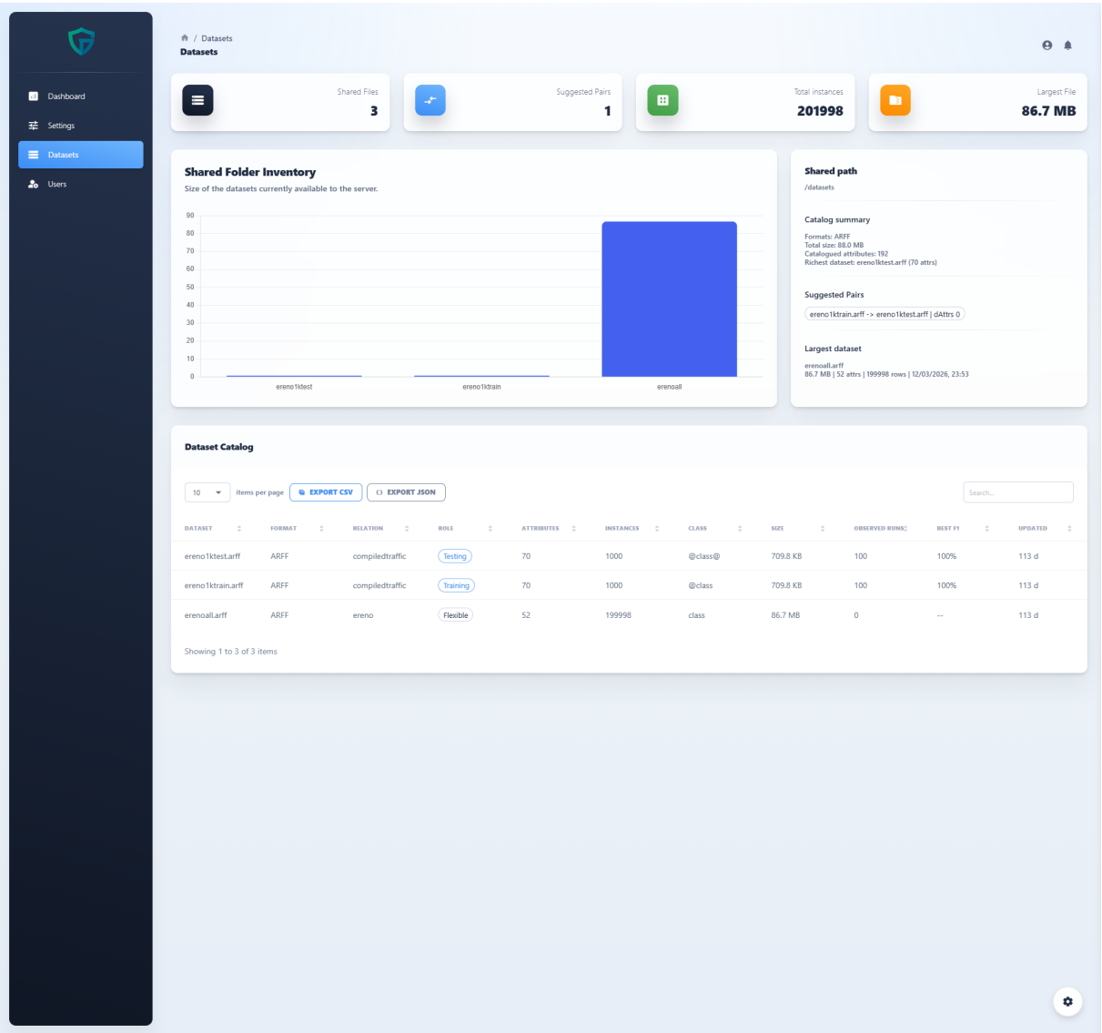
Figure 38 – Dataset list.
