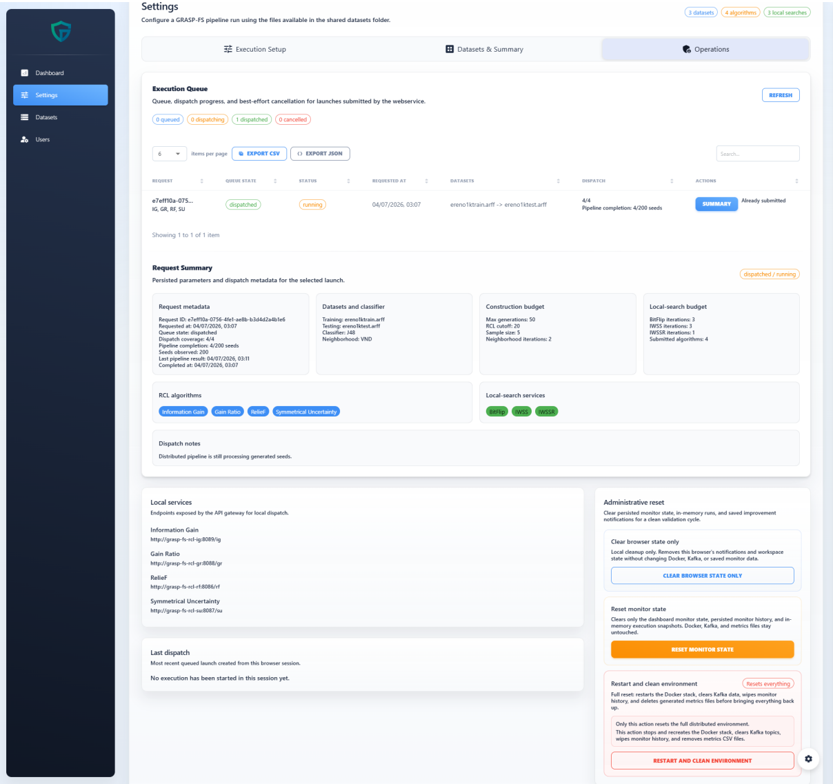
Figure 36 – Operations settings.
