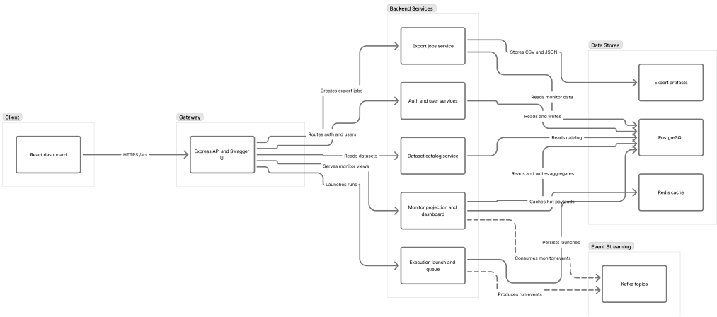
Figure 44 – Backend architecture of the system.
