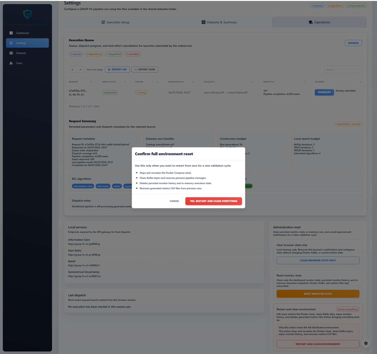
Figure 37 – Full reset dialog.
