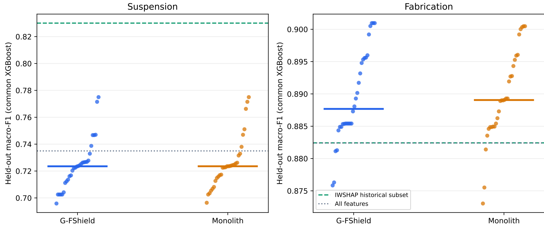
Figure 18 – Macro-F1 of frozen subsets under the common XGBoost protocol. Horizontal lines show the fixed all-feature and historical-IWSHAP-feature comparators.
