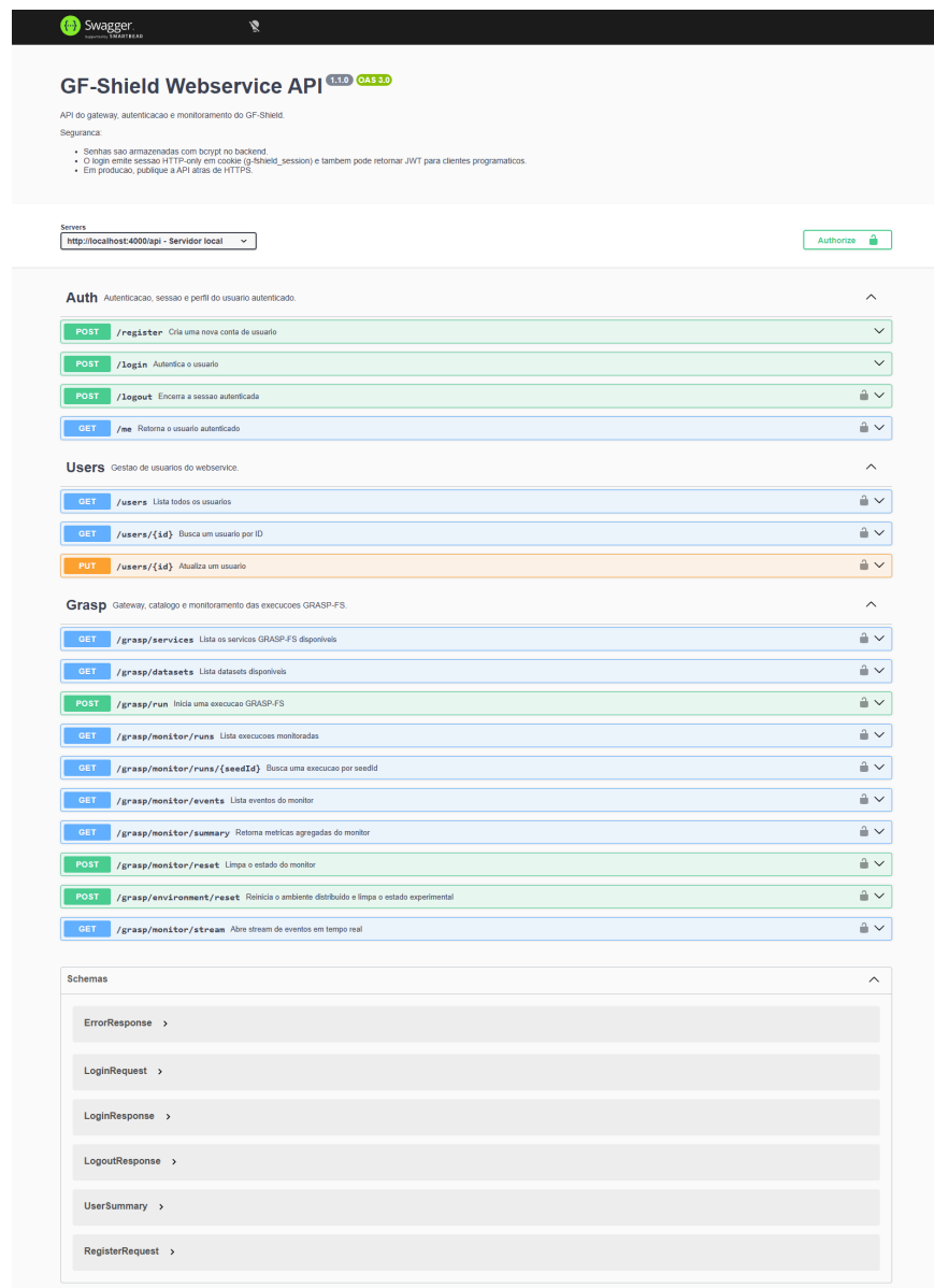
Figure 42 – Swagger documentation of the backend API.
