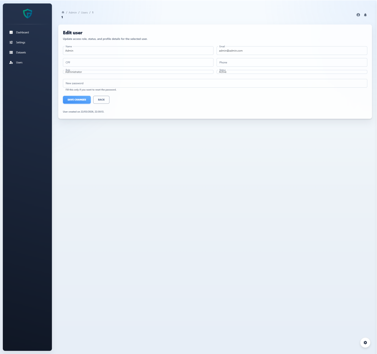
Figure 40 – User editing.
