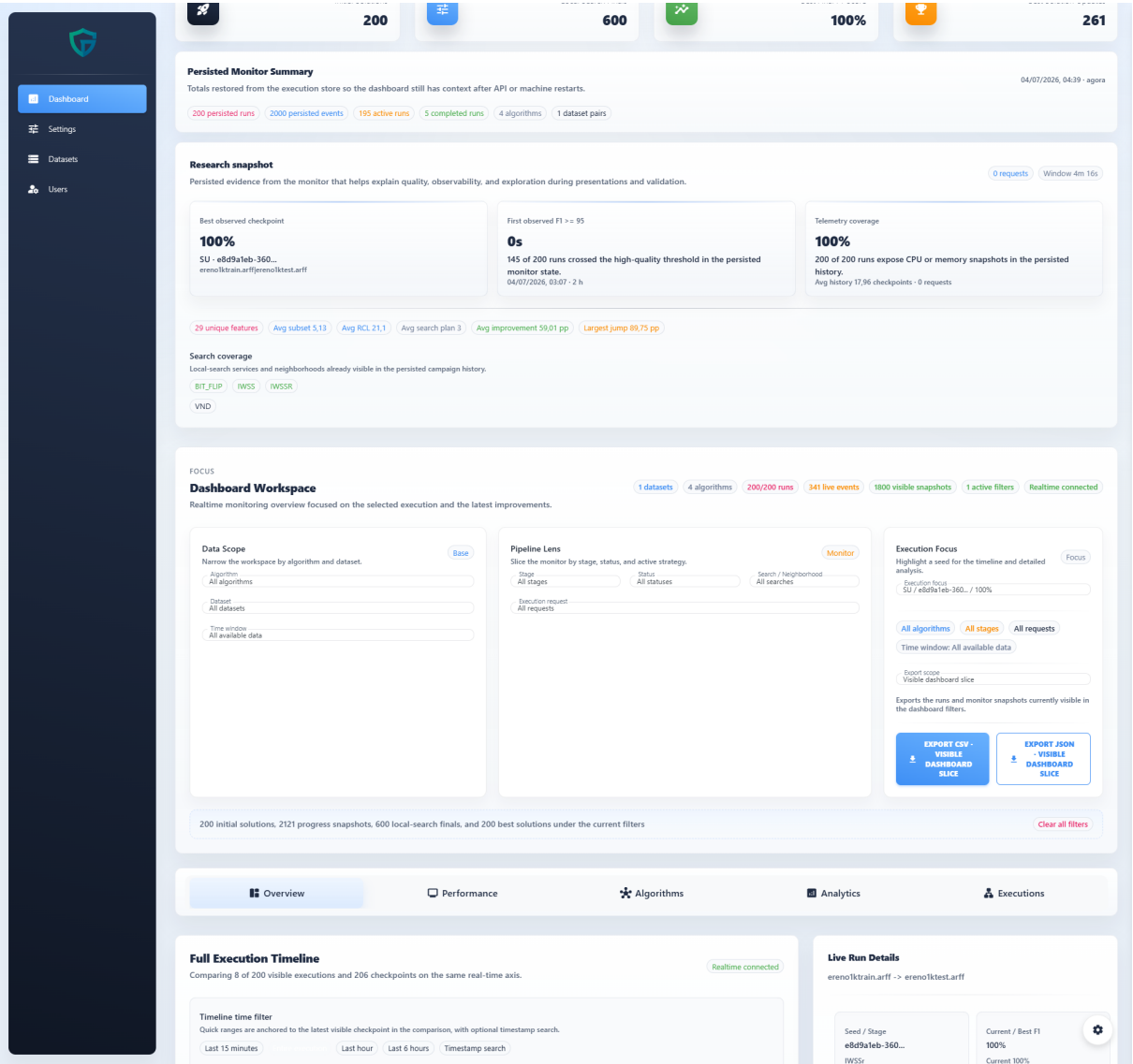
Figure 20 – Overview dashboard.
