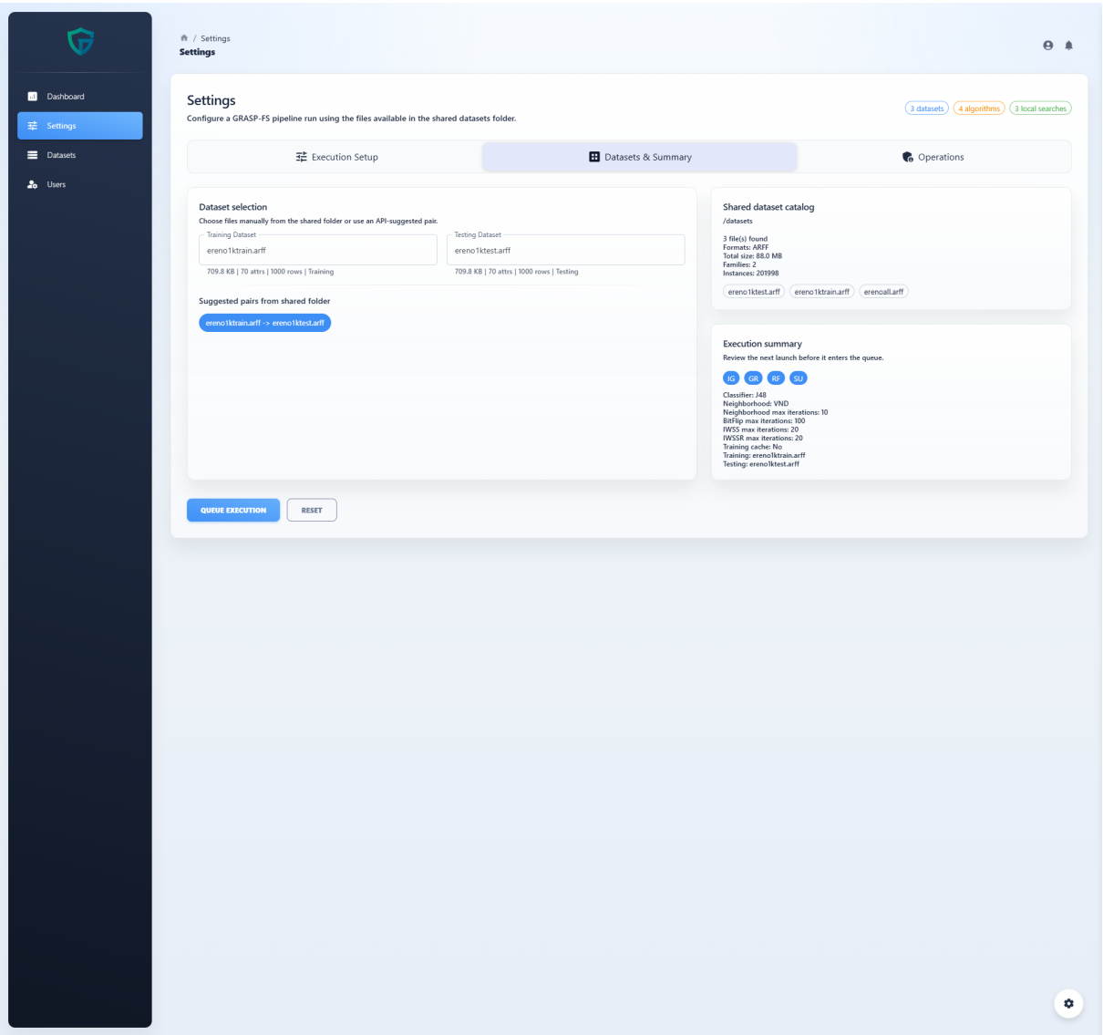
Figure 35 – Dataset settings.
