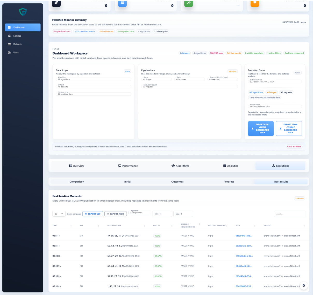
Figure 33 – Best solutions.
