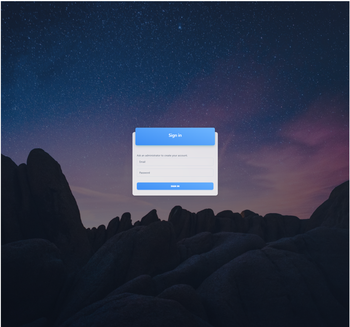
Figure 19 – Authentication screen.
