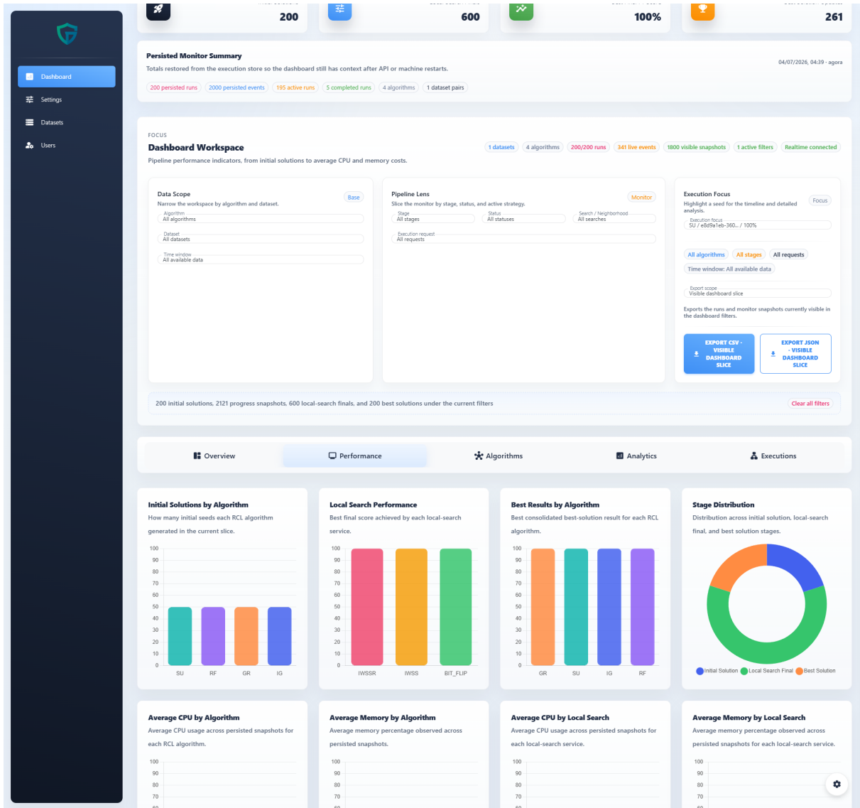
Figure 21 – Performance screen.
