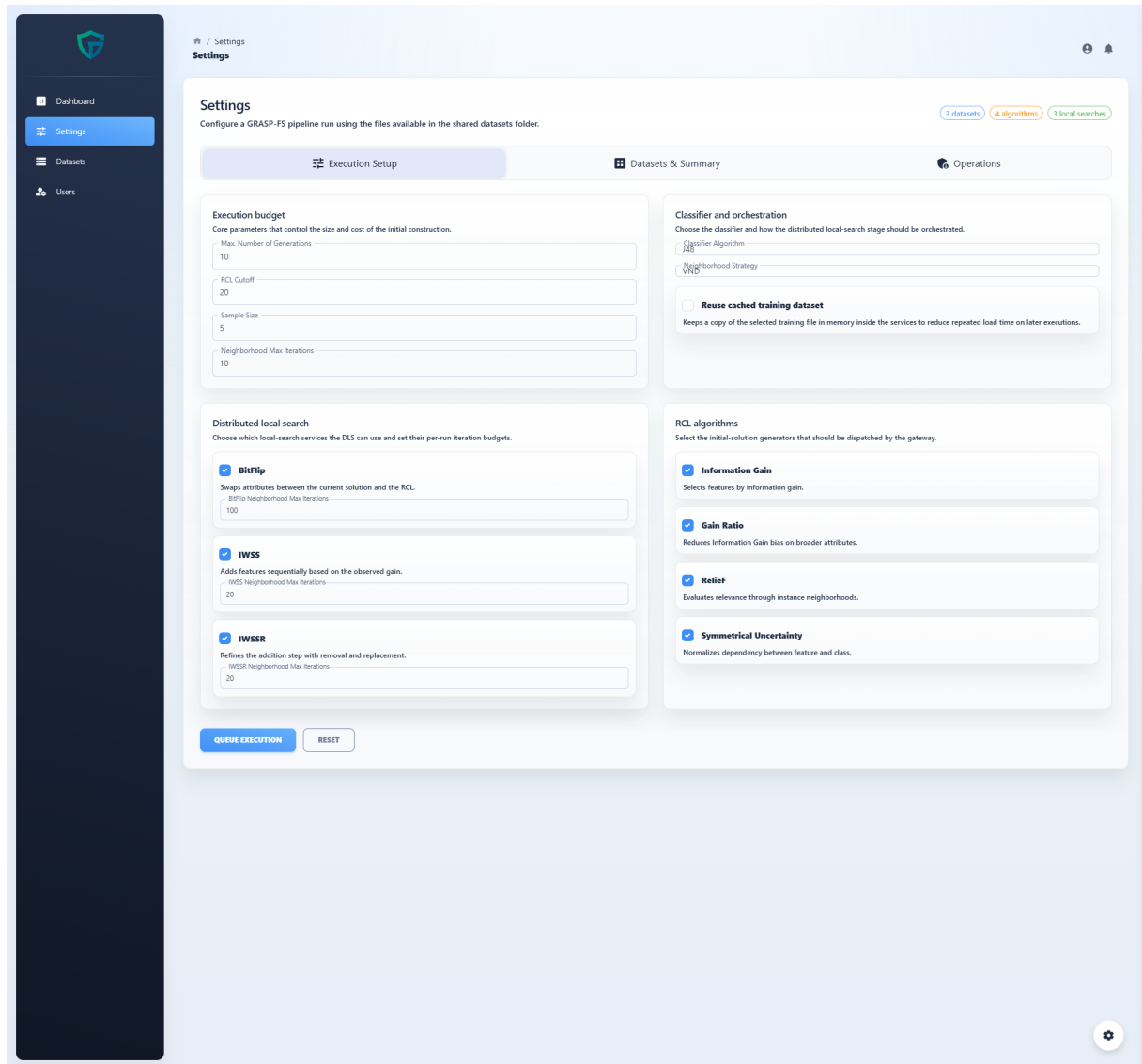
Figure 34 – Execution settings.
