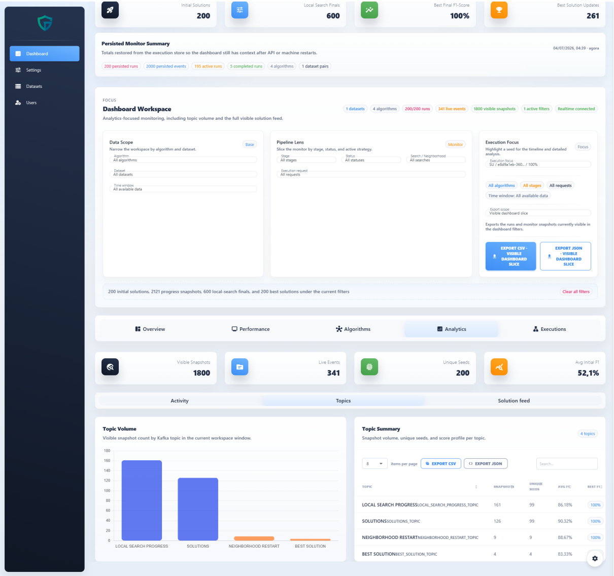
Figure 25 – Analytics topics.
