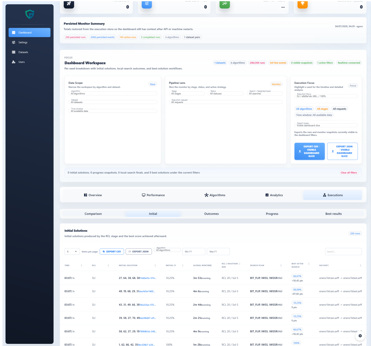
Figure 30 – Initial solutions.
