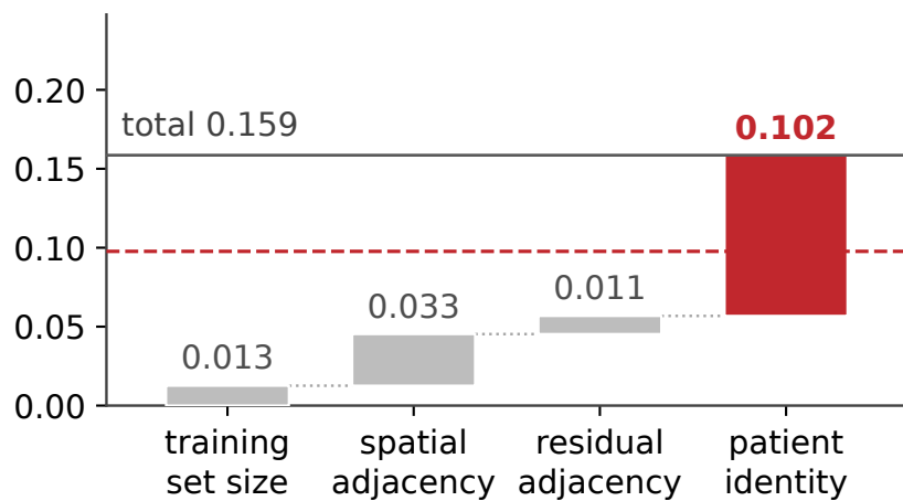
buffer removes the grid dependence
