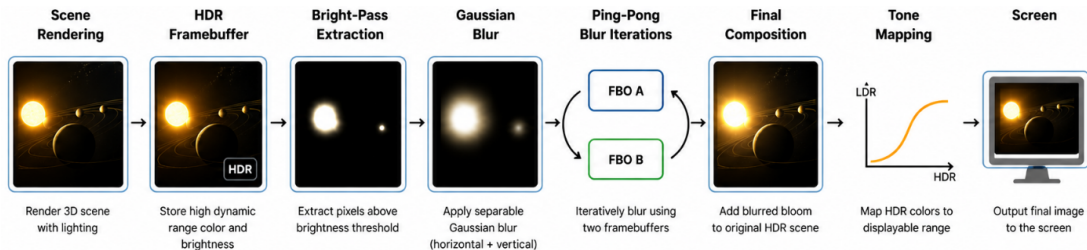
Figure: Entire Bloom Pipeline
