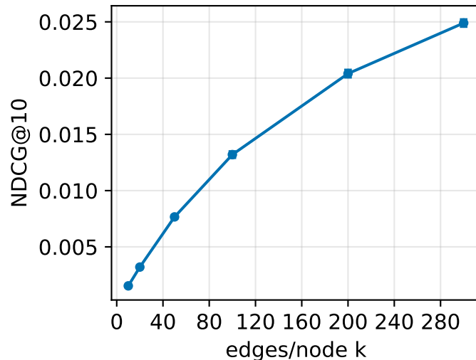
Decode-parameter sweeps: CDs
