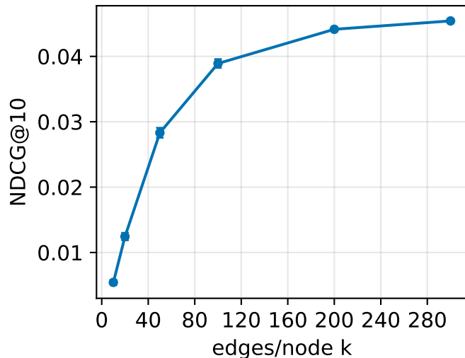
Decode-parameter sweeps: Toys
