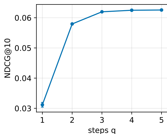
Figure 6 (README base, validation): Toys base b=200 , k=20 , q=3
