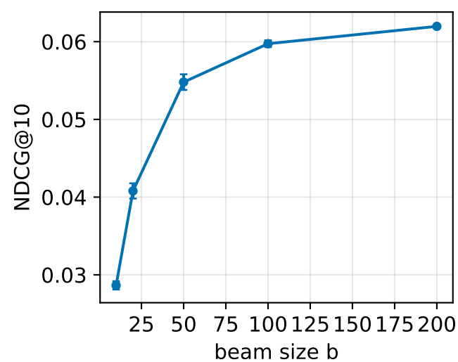
Figure 6 (README base, validation): Toys base b=200 , k=20 , q=3
