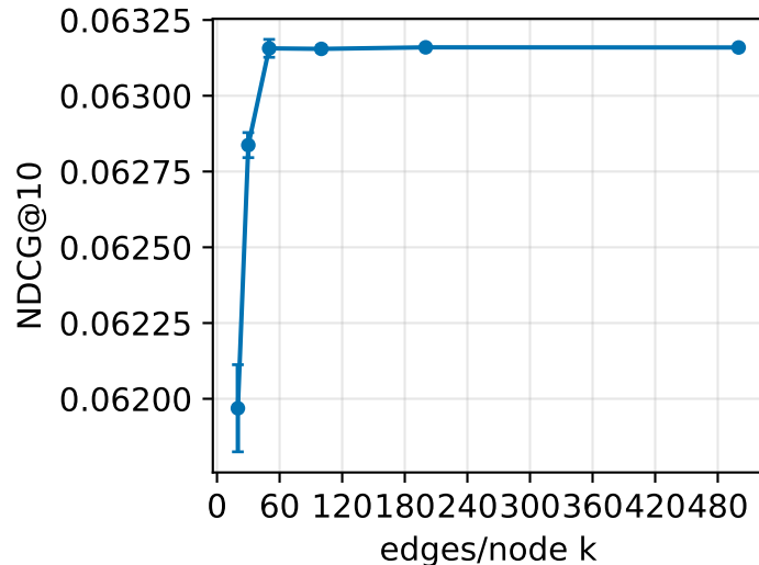
Figure 6 (README base, validation): Toys base b=200 , k=20 , q=3
