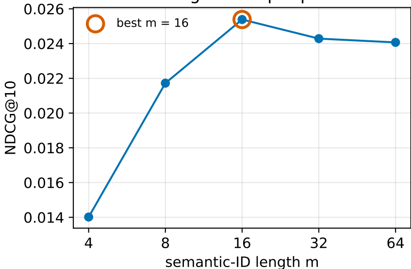
ID-length sweep: Sports
