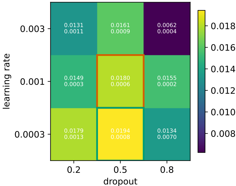
SASRec Sports NDCG@10 (b=2)
