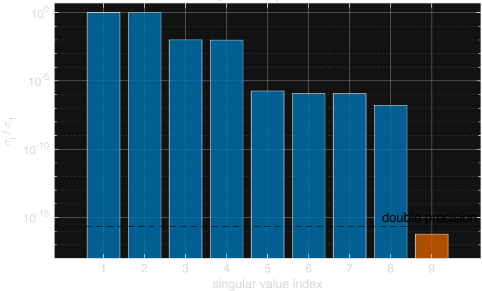
Controllability matrix spectrum: rank 8 of 9
