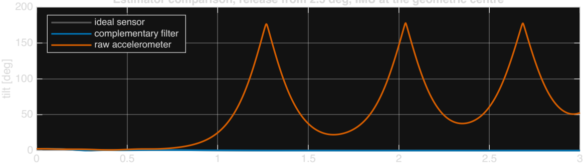
Estimator comparison, release from 2.5 deg, IMU at the geometric centre
