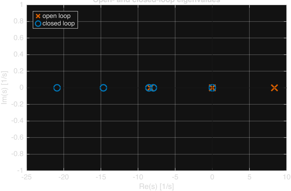
Open- and closed-loop eigenvalues
