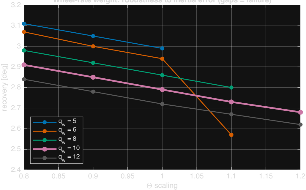
Wheel-rate weight: robustness to inertia error (gaps = failure)
