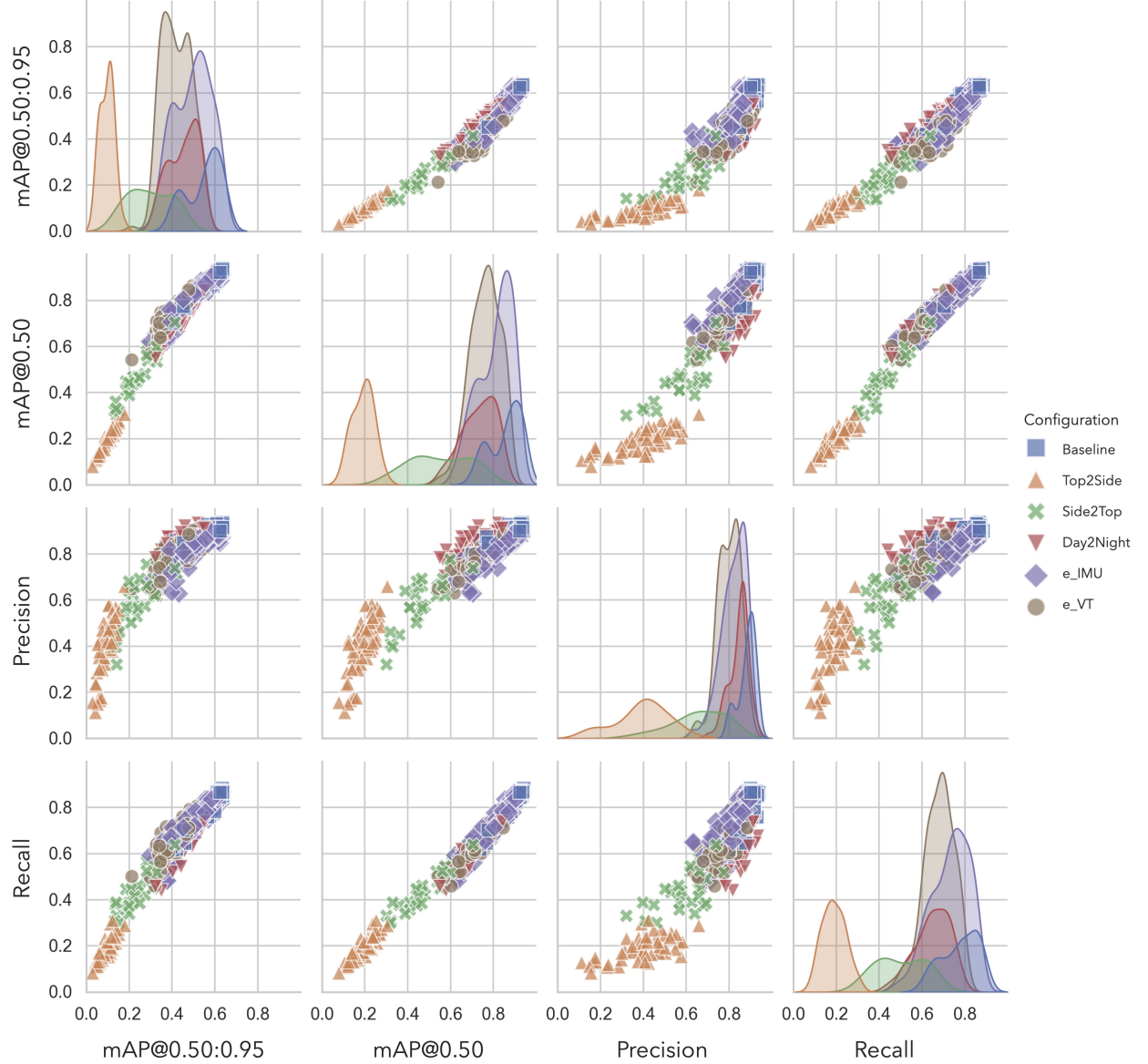
Figure 8: Pair-wise scatter plots illustrating the relationships among the four metrics used in this study. The metrics include mAP@0.5:0.95 , mAP@0.5 , precision, and recall. The diagonal panels show the distribution of each individual metric, while the off-diagonal panels display the correlation between each pair of metrics. In the scatter plots, each data point represents a single model evaluation iteration for a specific model size variant and data configuration. Different data configurations are distinguished by color. Only 500 iterations are shown for clarity.
