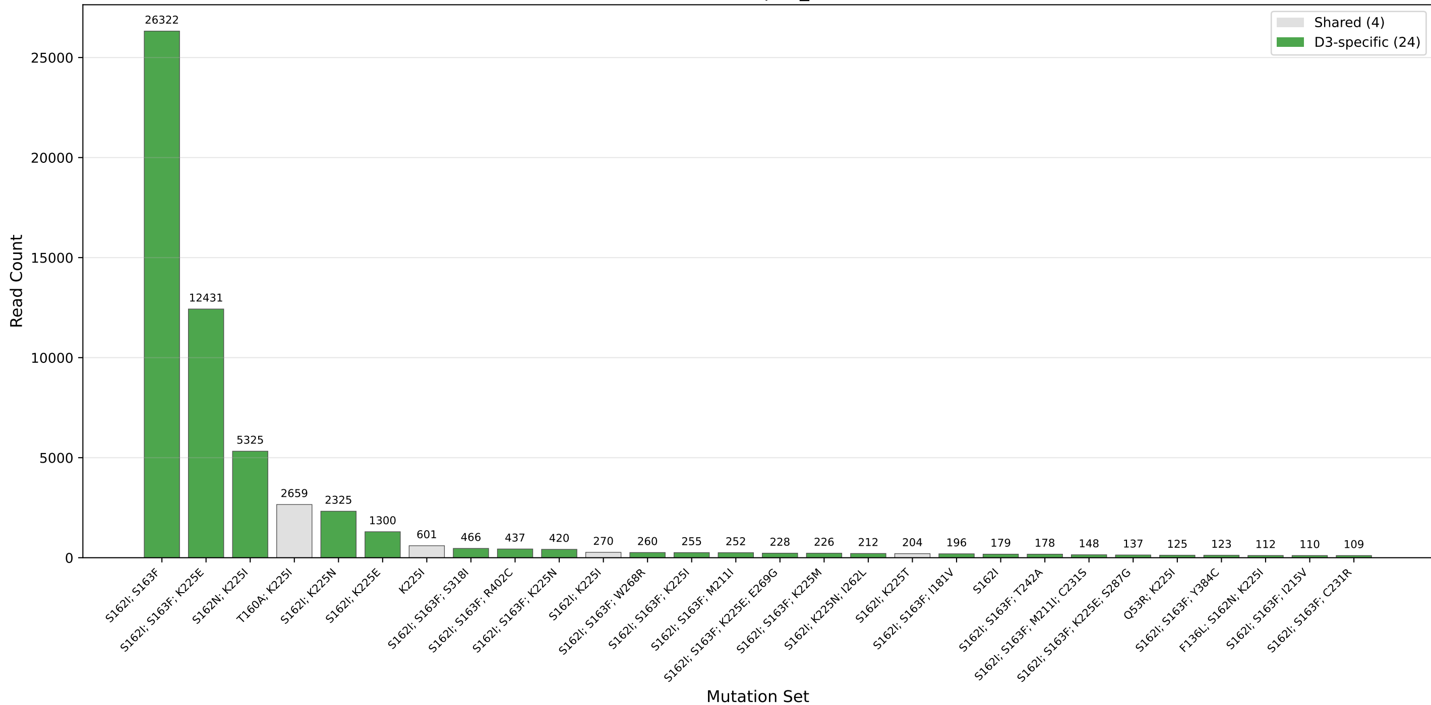
Mutation Sets with >100 Reads - A1 (Reference: sp23_dna.fa)
