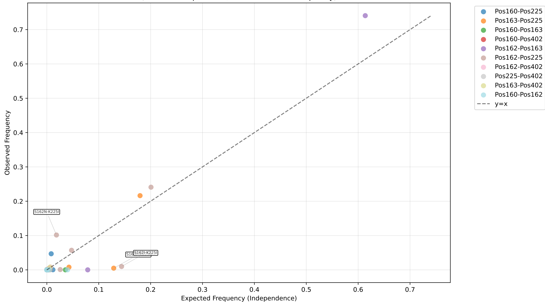
Observed vs Expected Mutation Pair Frequencies (DCA-filtered positions, >1.0% mutation frequency)
