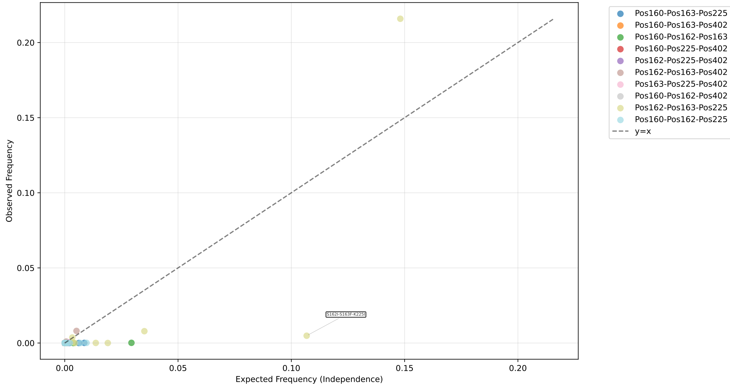
Observed vs Expected Mutation Triplet Frequencies (DCA-filtered positions, >1.0% mutation frequency)
