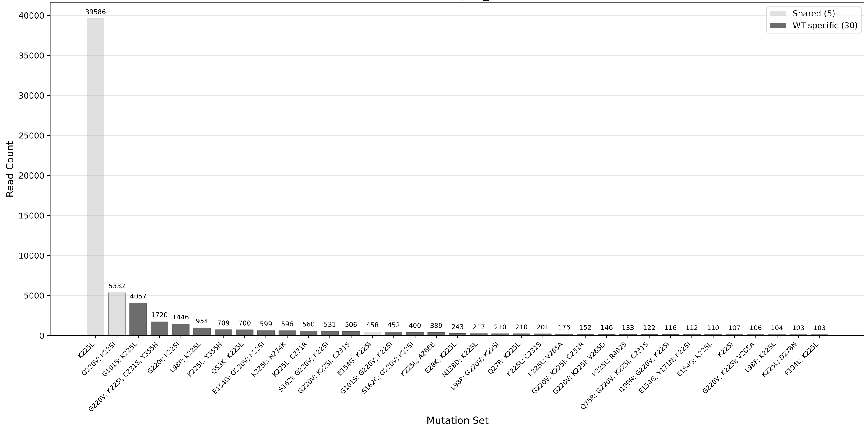
Mutation Sets with >100 Reads - D3 (Reference: sp24_dna.fa)
