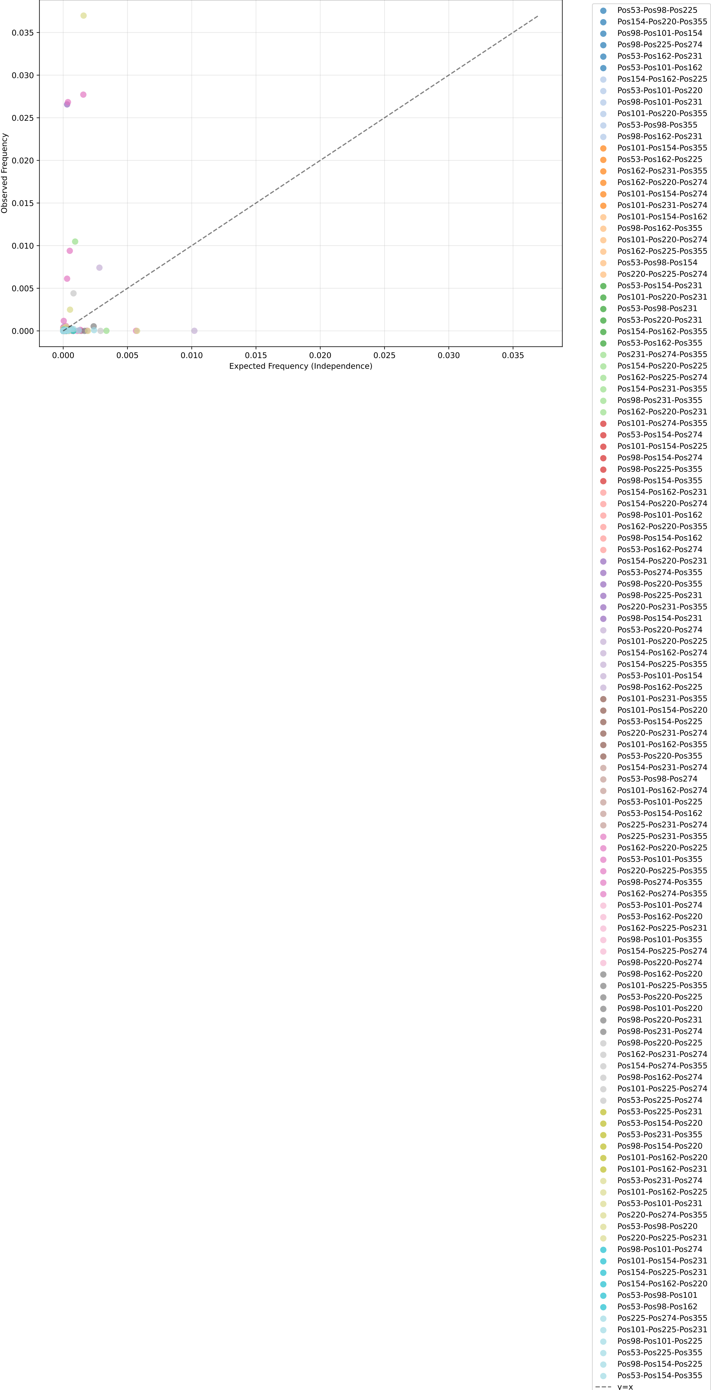
Observed vs Expected Mutation Triplet Frequencies (DCA-filtered positions, >1.0% mutation frequency)
