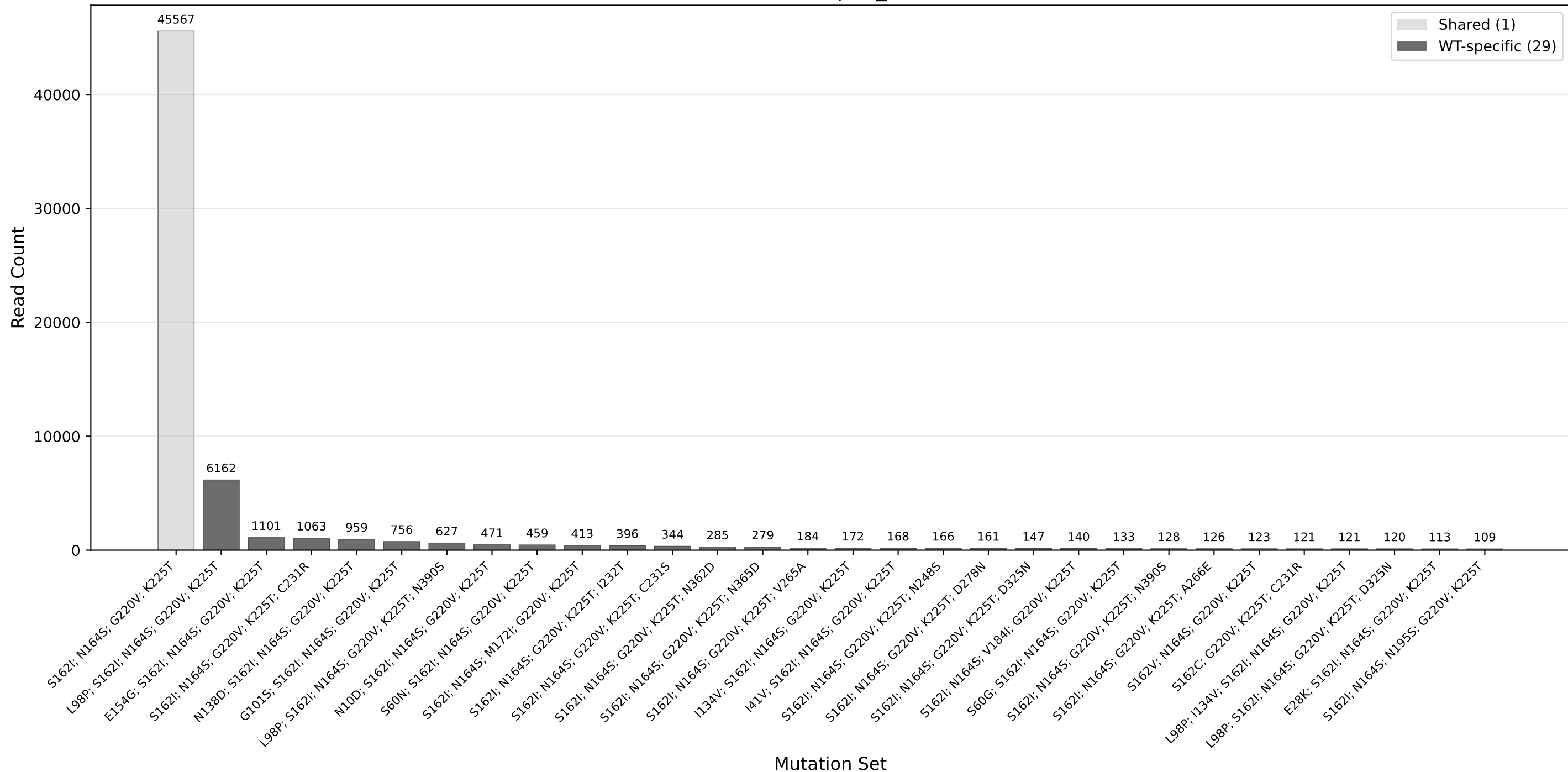
Mutation Sets with >100 Reads - F3 (Reference: sp24_dna.fa)
