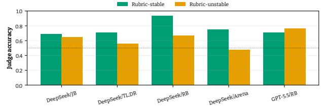
Figure 2: Judge accuracy on rubric-stable (green) vs. rubric-unstable (orange) subsets, per judge–benchmark pair; the dotted line marks chance (0.5). The stable–unstable gap is positive for the mid-band judge and shrinks or reverses for the frontier judge (analyzed in §4.2).
