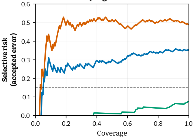
JudgeBench
