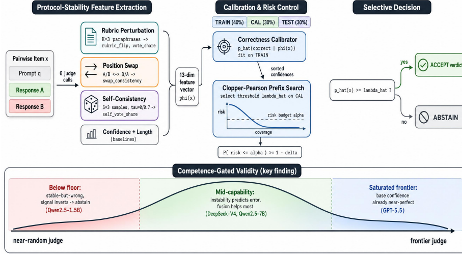
Figure 1: Overview of CARE-Judge. Six judge calls per item yield three protocol-stability feature families (rubric perturbation, position swap, self-consistency) plus confidence/length baselines ( \phi(x) ); a correctness calibrator fit on TRAIN and an exact Clopper–Pearson threshold \hat{\lambda} selected on CAL drive an accept/abstain decision on held-out TEST. Key finding (bottom): the signal is competence-gated —it inverts below a competence threshold (abstain), helps most in the mid-capability band, and is redundant for a saturated frontier judge.
