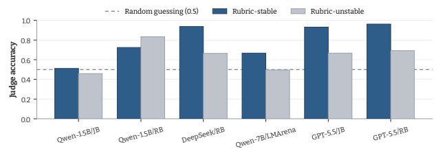
Figure 2: Judge accuracy on rubric-stable (blue) vs. rubric-unstable (grey) subsets, ordered by judge accuracy; the dashed line marks chance (0.5). For the mid-accuracy and frontier judges the stable subset is clearly more accurate, so stability is informative. For the below-competence Qwen2.5-1.5B, both subsets sit near chance and stability no longer separates correct from incorrect verdicts (analyzed in §4.2, §4.4).
