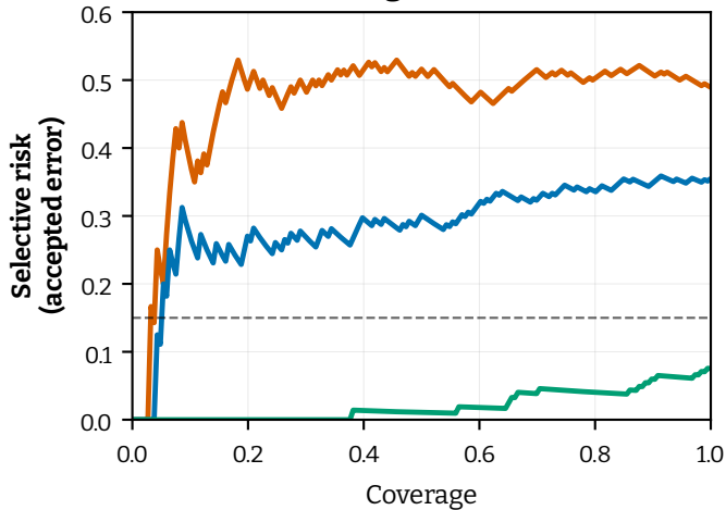
JudgeBench
