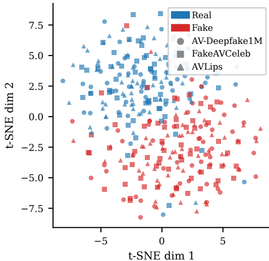
Manipulation factor H^m (colored by real/fake)
