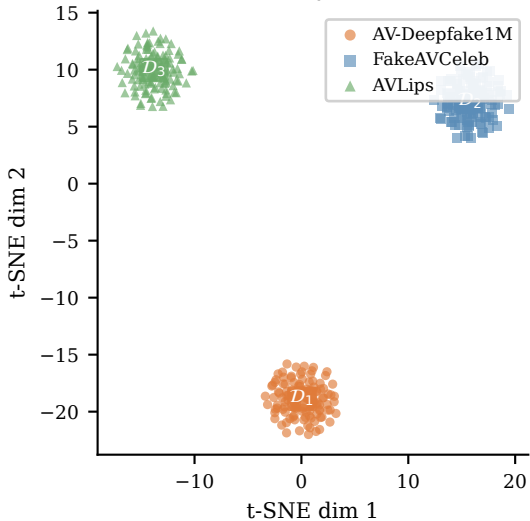
Domain factor H^d (colored by dataset)
