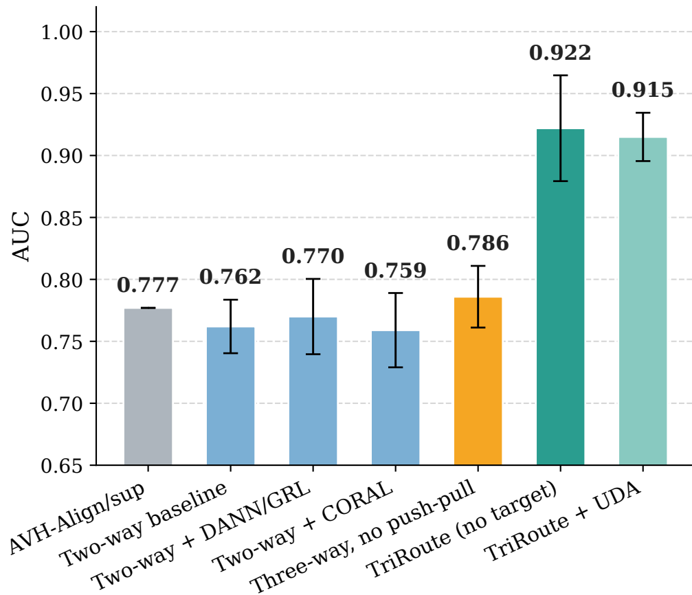
Overall AUC
