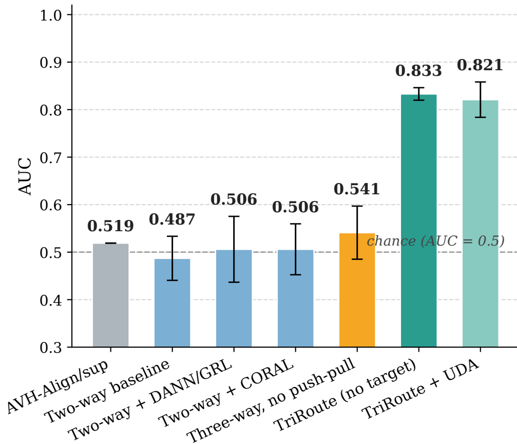
FakeVideo-RealAudio (FV-RA)
