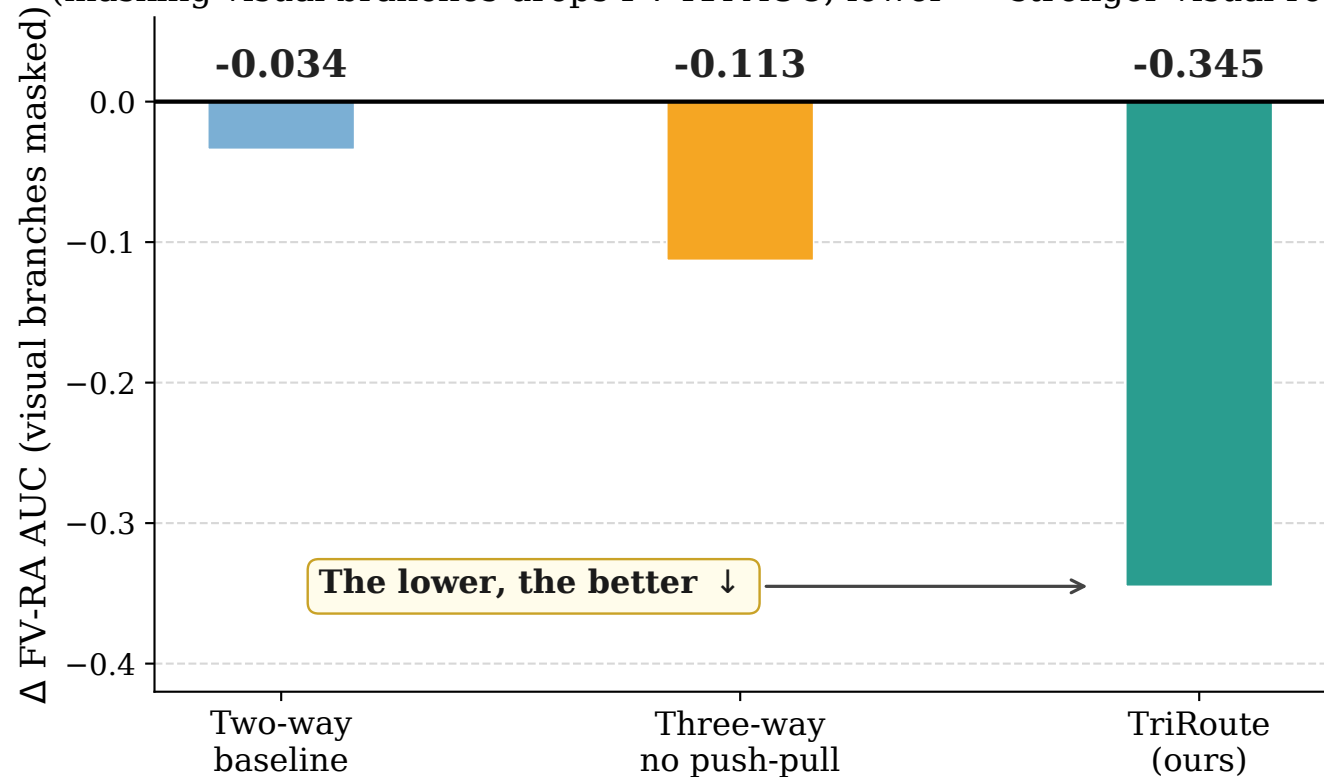
Head Ablation: Routing Dependence on Visual Branches (masking visual branches drops FV-RA AUC; lower = stronger visual routing)
