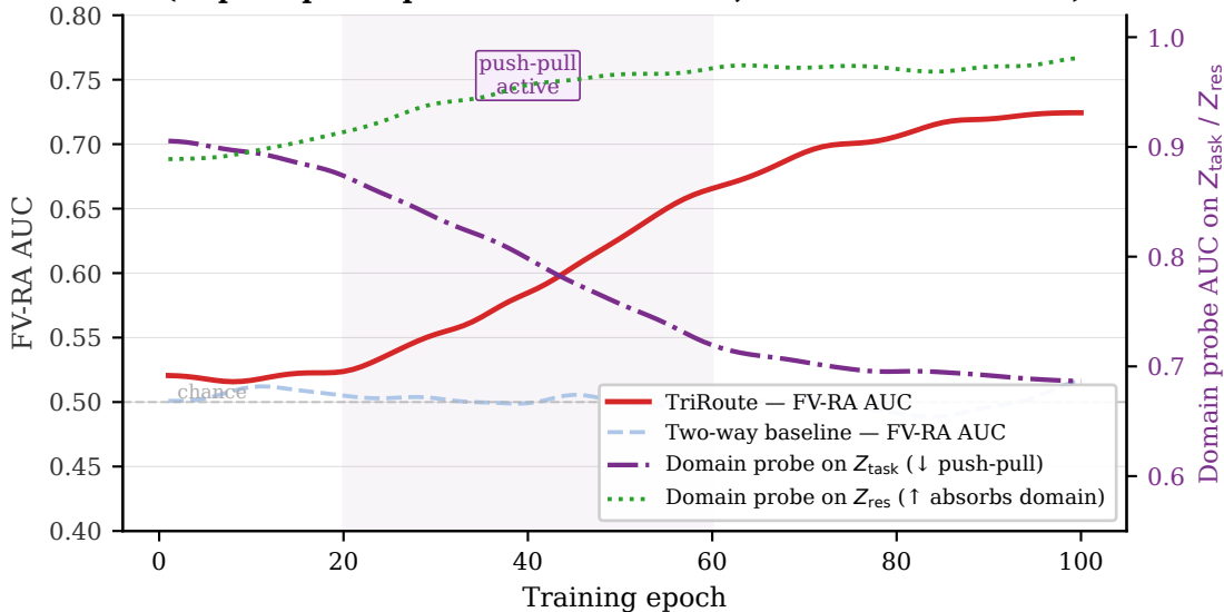
Training dynamics: FV-RA gain vs. domain suppression (as push-pull expels domain shortcuts, visual-fake AUC rises)
