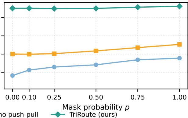
Audio masking (FV-RA \uparrow if audio was a distractor)
