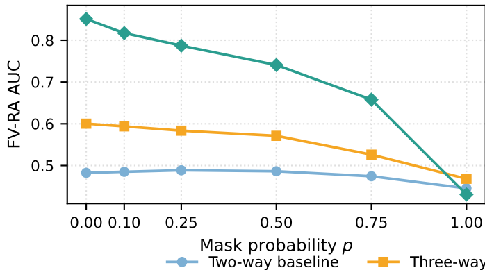
Visual masking (FV-RA \downarrow if routing through vision)
