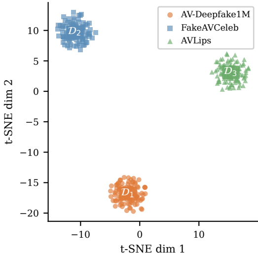
Residual factor Z_{\text{res}} (colored by dataset)
