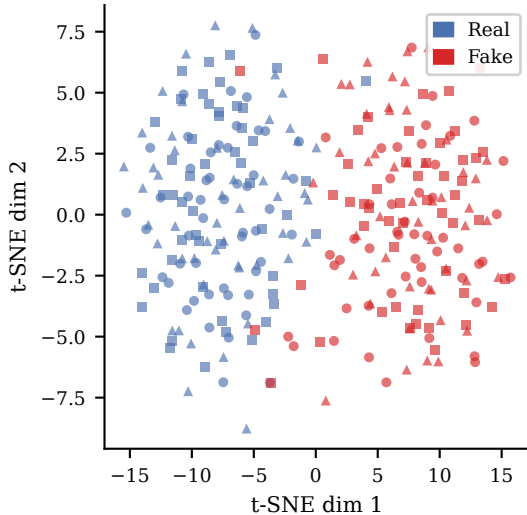
Task factor Z_{\text{task}} (colored by real/fake)
