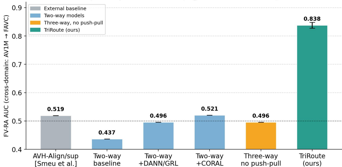
Cross-Domain FakeVideo-RealAudio Detection (FV-RA requires visual evidence; higher = more visual reliance)
